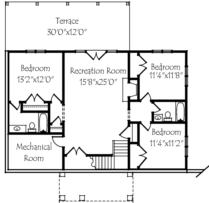
TERRACE LEVEL FLOOR PLAN
